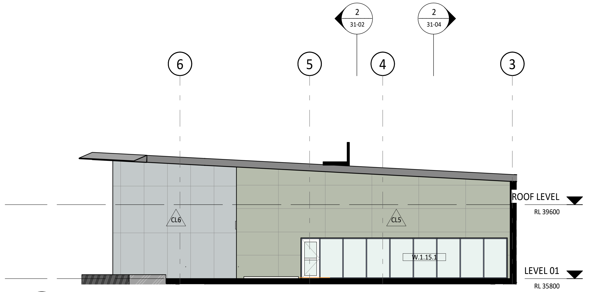
3 EAST ELEVATION 2 21-10 1 : 100
