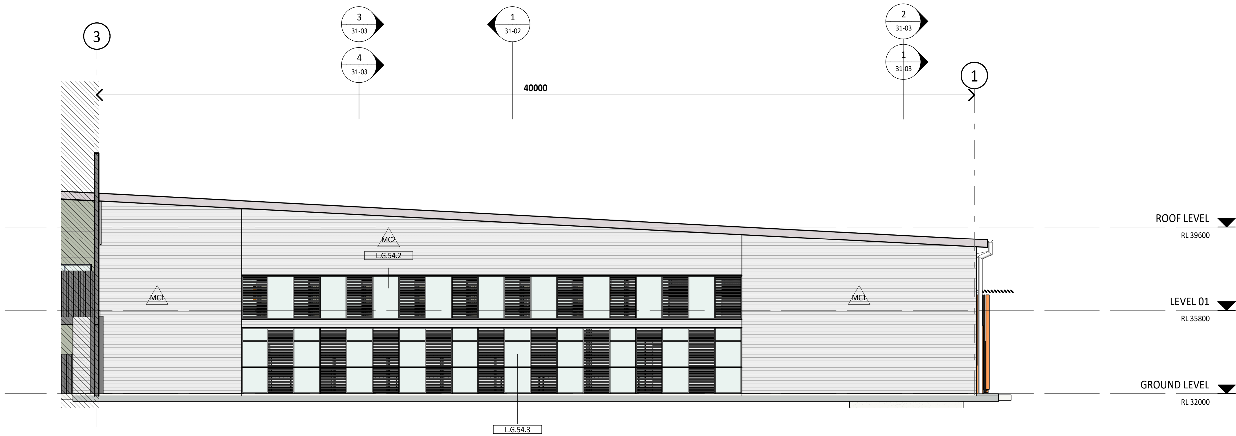
2 BUILDING ELEVATION - EAST - 2 21-00 1 : 100
