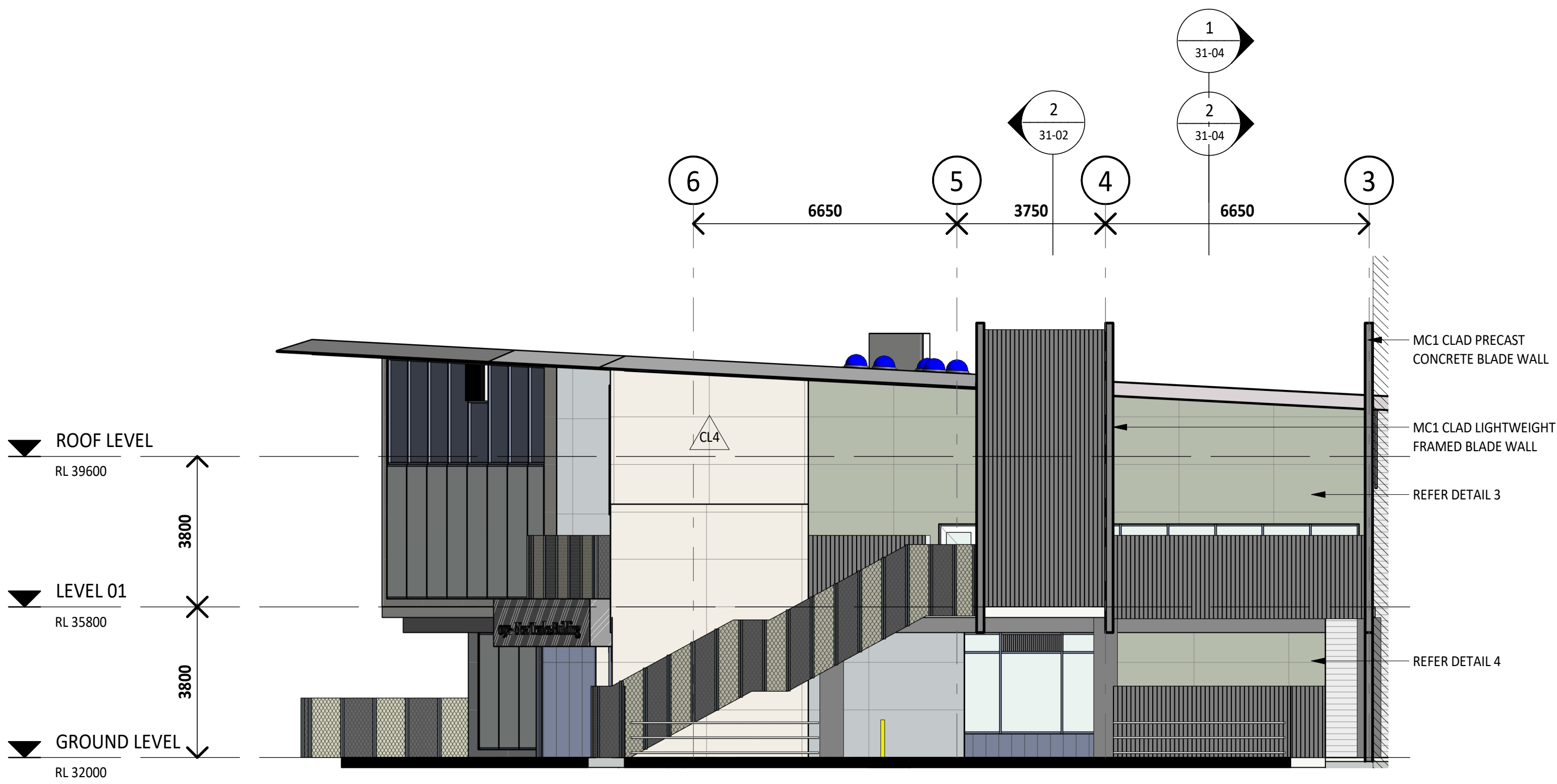
1 BUILDING ELEVATION - EAST - 1 21-00 1 : 100
