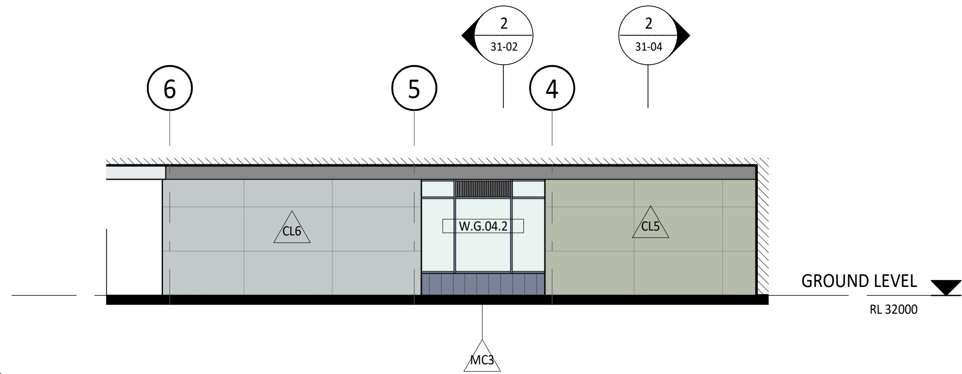
4 EAST ELEVATION 3 21-00 1 : 100
